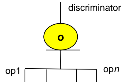
partial/overlapping
