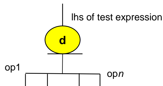
partial/disjoint
