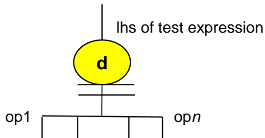
total/disjoint
