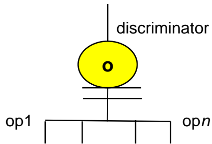
total/overlapping
